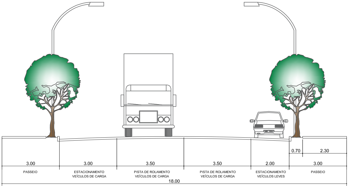
VIA ARTERIAL PRINCIPAL E VIA ARTERIAL SECUNDÁRIA
